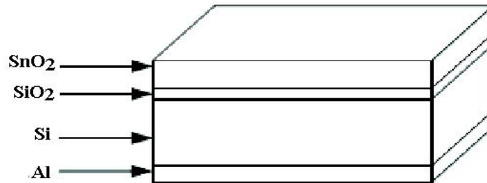
Fig. 1: Schematic diagram of the fabricated MIS solar cells
