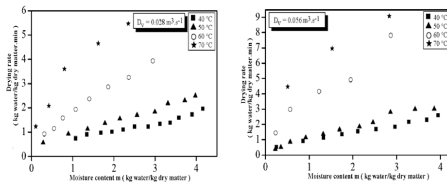
Fig. 7: Variations of drying rate as a function of moisture content for different air-drying temperature of mint leaves ( M. pulegium )
