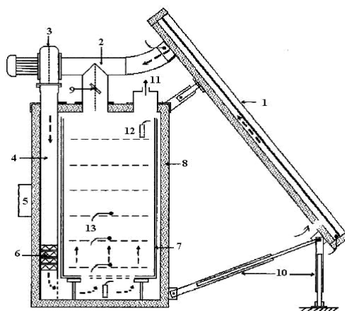
Fig. 2: Schematic representation of the solar dryer (1) Solar collector; (2) Circulation fan; (3) Fan; (4) Air flow direction; (5) Control box; (6) Auxiliary heating system; (7) Shelves; (8) Drying cabinet; (9) Recycling air; (10) Control foot; (11) Exit of air; (12) Humidity probes; (13) Thermocouples
