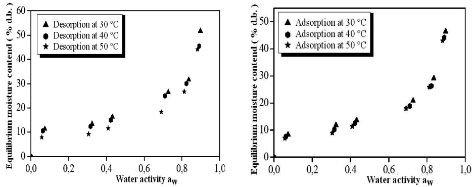
Fig. 3: Influence of temperature on the equilibrium moisture content of mint leaves ( M. pulegium )
