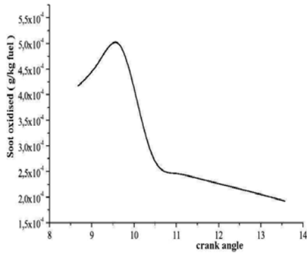
Fig. 6: Soot oxidised (g/kg fuel)
